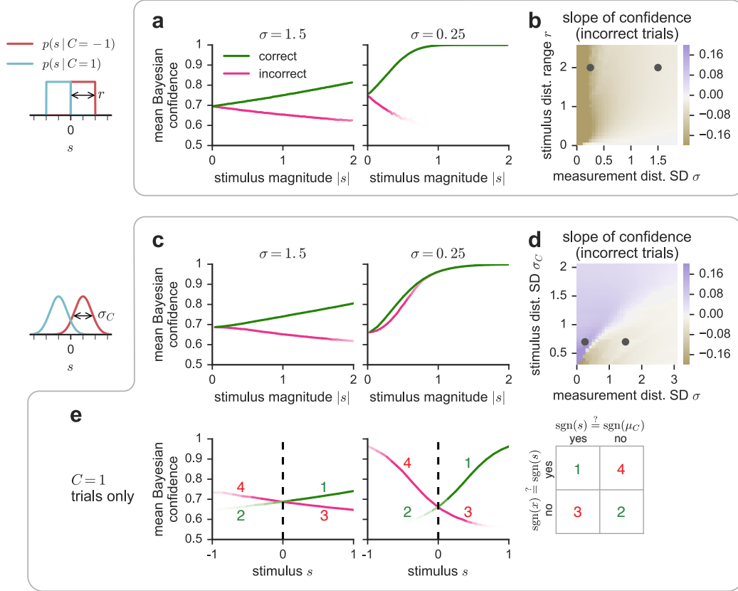
Figure 2.3 The divergence signature is not a necessary condition for Bayesian confidence. For two stimulus distribution types, we simulated 2 million trials. (a) With uniform stimulus distributions defined by p(s | C = 1) = \mathcal{U}(s; 0, 2) , the divergence signature is predicted under both high- and low-noise regimes. The fadedness of the line indicates conditions for which there are few trials. (b) Heatmap indicates the slope of the pink lines in a . At all values of \sigma and distribution range, the slope is negative. Slopes were obtained by generating binned mean confidence values as in a and fitting a line to those values. Black markers indicate the parameters used in a , with left dot corresponding to right plot and conversely. (c) With Gaussian stimulus distributions defined by p(s | C = 1) = \mathcal{N}(s; 1, \sigma_C = 0.7) , the divergence signature appears only when measurement noise is high, i.e., when \sigma \lesssim 0.6 . (d) As in b but for Gaussian distributions with means of \pm 1 . Under some values of \sigma and \sigma_C , the slope is positive, indicating that the divergence signature is not a necessary condition for Bayesian confidence. (e) Visual explanation for why, under Gaussian stimulus distributions, the divergence signature appears only at relatively high \sigma values. Plots represent the same data as in c , but over s instead of |s| . For clarity, we only use trials drawn from category C = 1 ; the argument is unaffected. Incorrect trials fall into two categories: on trials in which s is positive but x is negative due to noise, confidence goes down as |s| increases (branch 3); on trials in which s and x are both negative, confidence increases with |s| (branch 4). At high levels of noise, branch 3 has more trials than branch 4, and dominates the averaging that occurs when plotting trials from both categories over |s| . At low levels of noise, branch 4 instead dominates, and the divergence signature disappears. Note that, for non-overlapping distributions (e.g., those in a, b ), there are no trials in which s has a different sign than the stimulus distribution mean, so branches 2 and 4 do not exist, and the divergence signature is always present.
