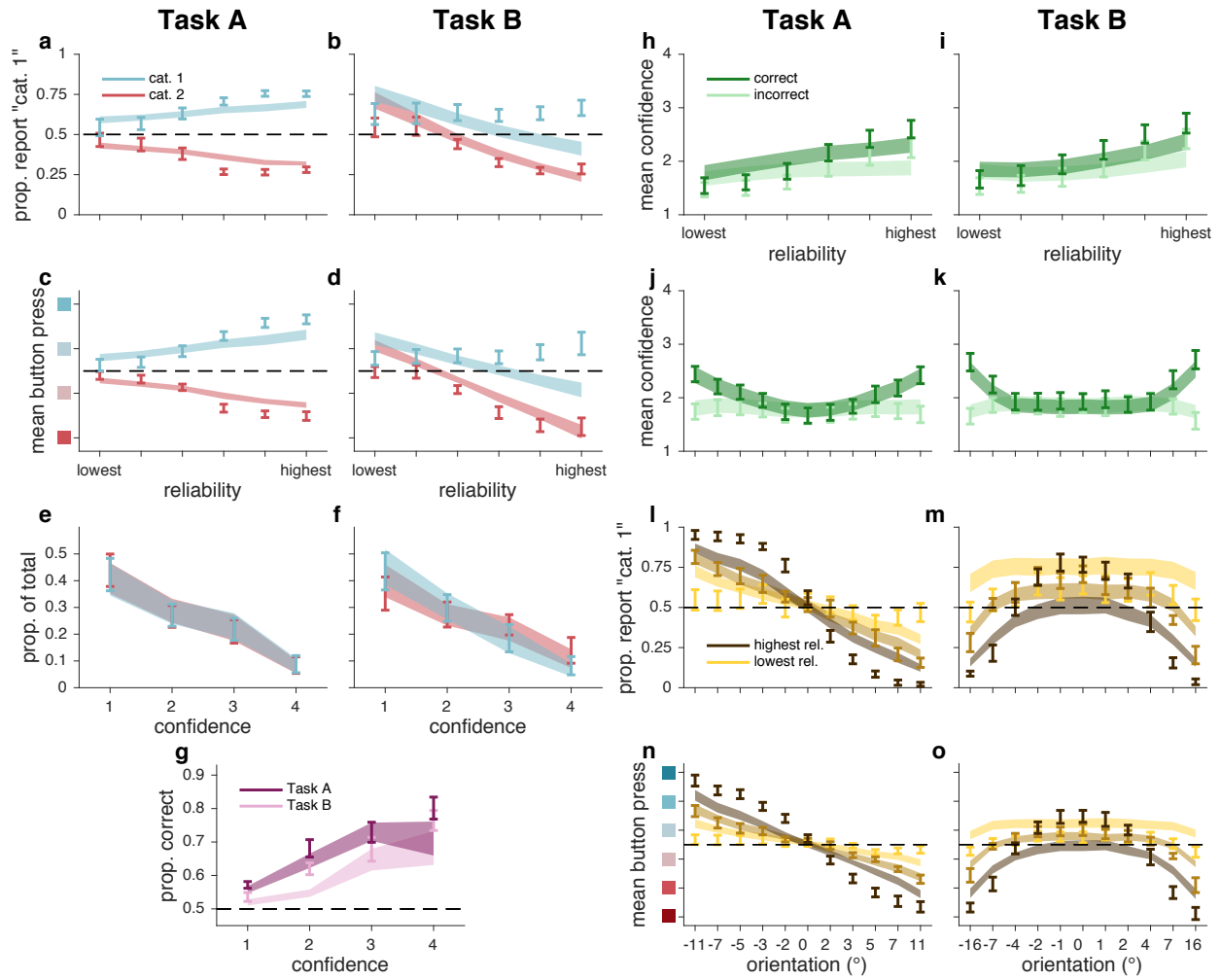
Figure 3.23 Orientation Estimation fits, as in Figure 3.8.
