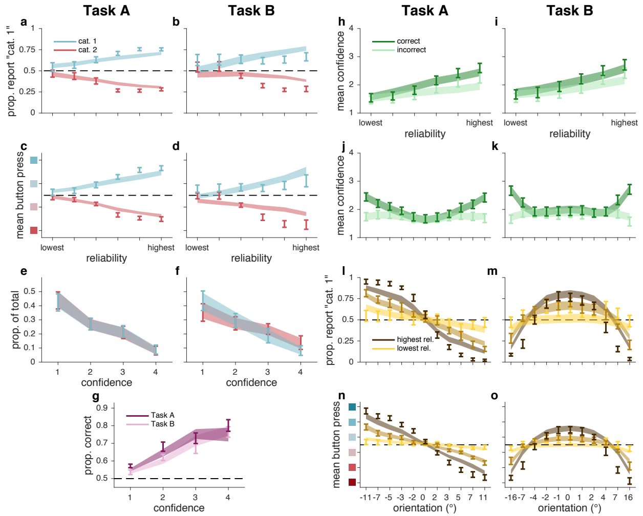
Figure 3.21 Bayes- dN fits, as in Figure 3.8
