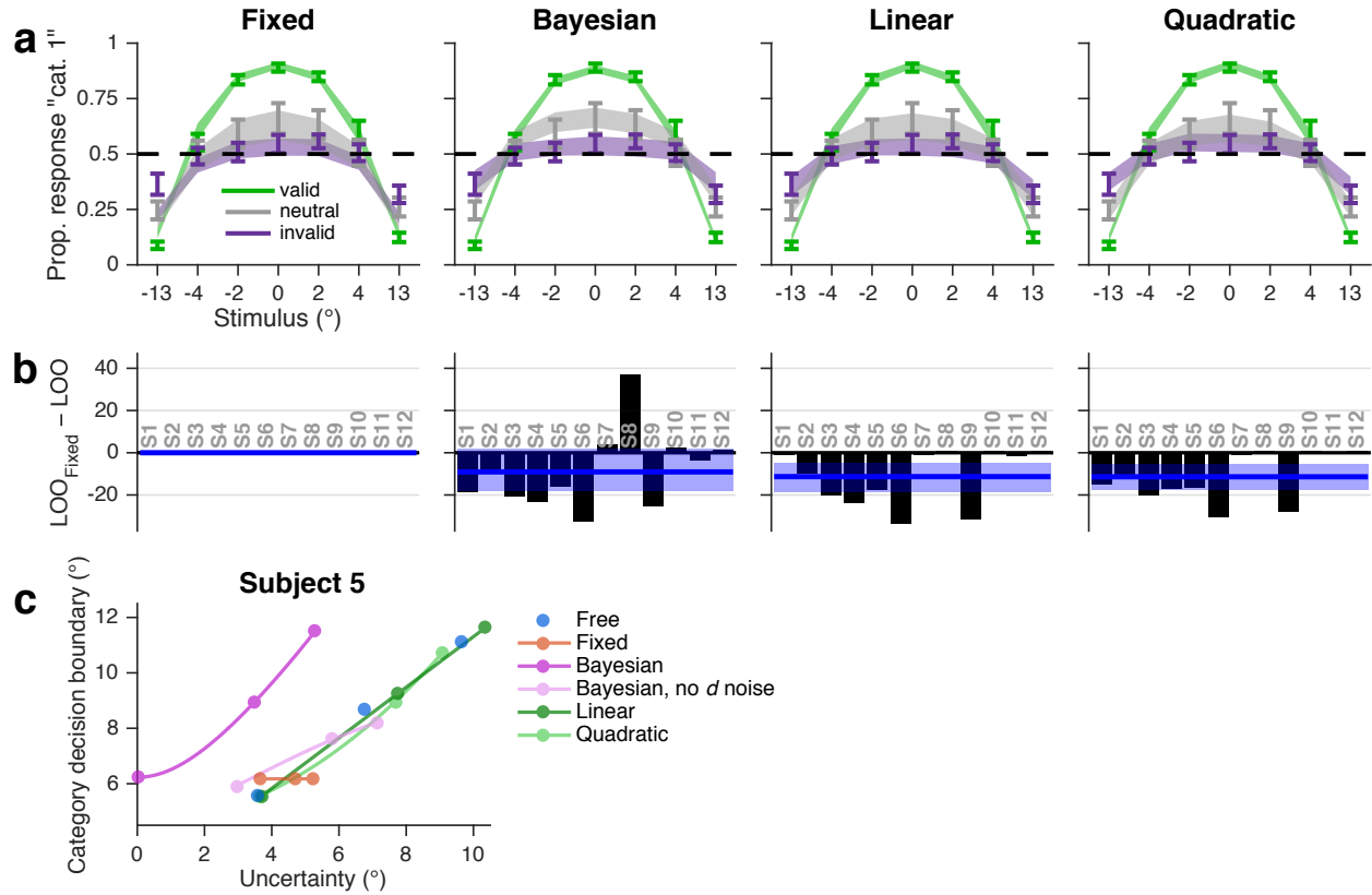
Figure 4.7 Category choice-only models. (a) Proportion of category 1 responses as a function of orientation and cue validity. Error bars show mean and SEM across subjects. Shaded regions are mean and SEM of model fits (Methods). (b) LOO model comparison, as in Figure 4.5c. (c) Mean MCMC orientation uncertainty and category choice boundary parameter estimates for a representative subject. Estimates are plotted as a function of attention condition (valid, neutral, invalid; filled circles), along with their generating functions (curves), for the four main models fit to the category choice data only, plus a Bayesian model with no noise on the decision variable d and a nonparametric model in which choice boundaries are unconstrained (Free; parameter estimates from this model are plotted in gray for all subjects in Figure 4.8). The Bayesian curve is to the left of the other curves, because noise attributed to orientation uncertainty in the other models is partially attributed to decision noise in the Bayesian model; when the decision noise parameter is removed (Bayesian, no d noise), the curve aligns with the others.
