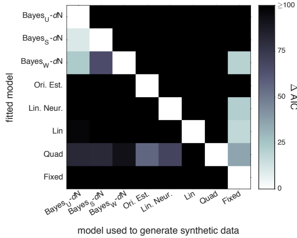
Figure 3.26 Model recovery analysis. Shade represents the difference between the mean AIC score (across datasets) for each fitted model and for the one with the lowest mean AIC score. White squares indicate the model that had the lowest mean AIC score when fitted to data generated from each model. The squares on the diagonal indicate that the true generating model was the best-fitting model, on average, in all cases.
