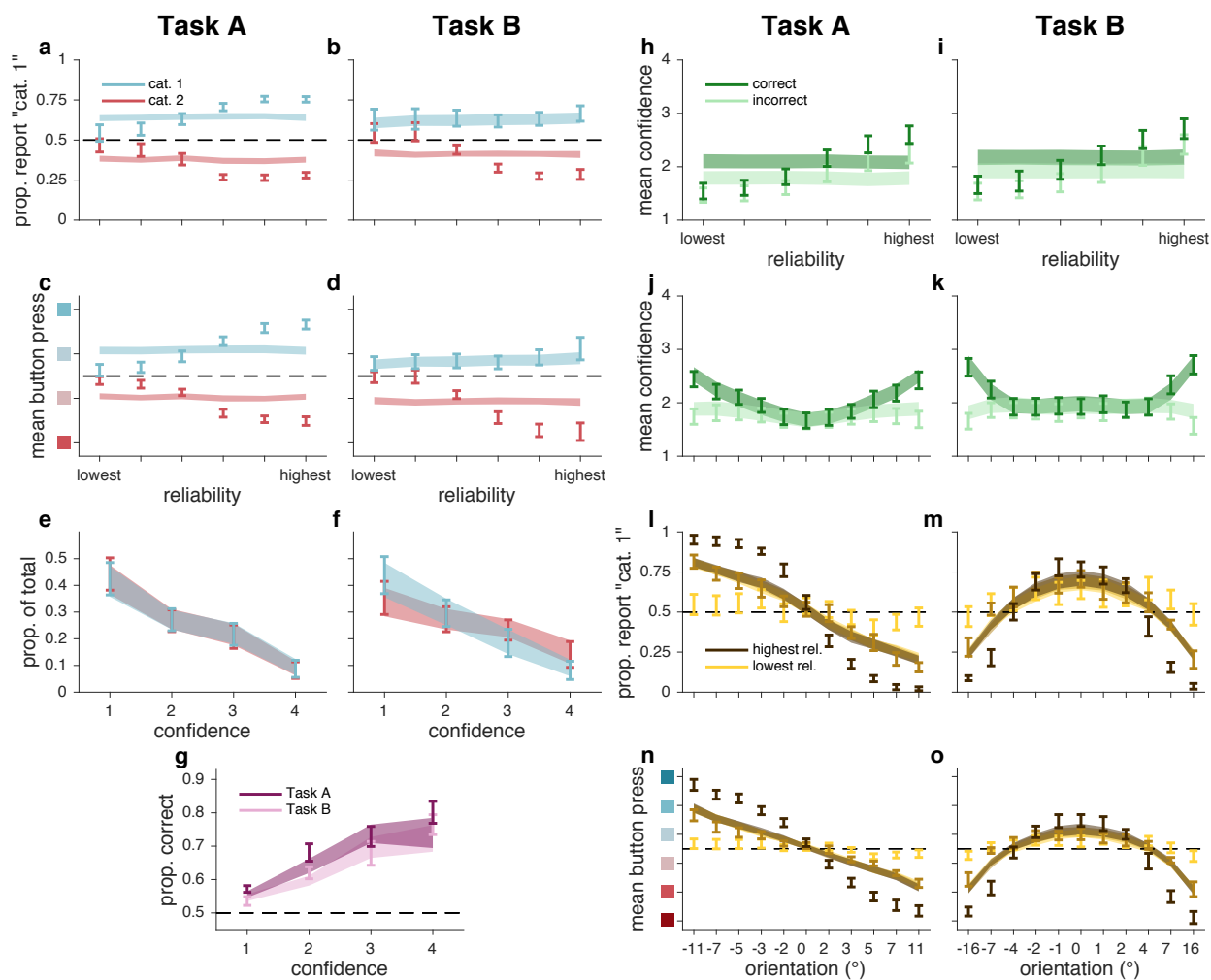
Figure 3.22 Fixed fits, as in Figure 3.8.
