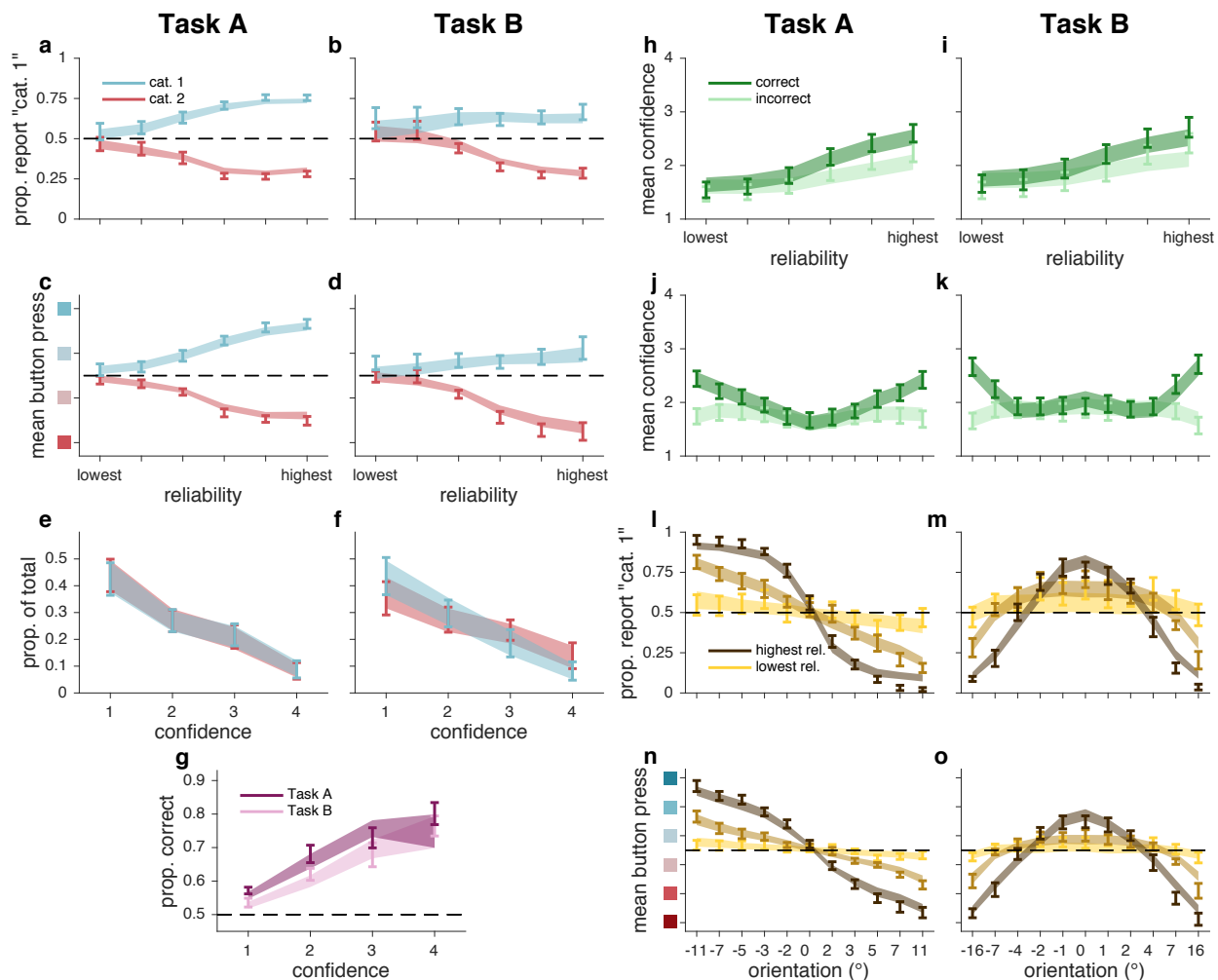
Figure 3.25 Lin fits, as in Figure 3.8.
