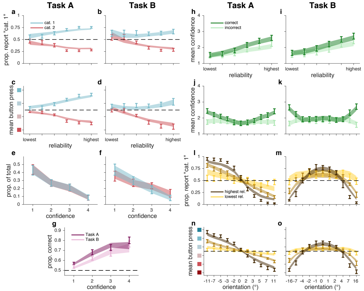
Figure 3.8 Behavioral data and fits from best model (Quad), experiment 1. Error bars represent \pm 1 s.e.m. across 11 subjects. Shaded regions represent \pm 1 s.e.m. on model fits (). (a,b) Proportion “category 1” reports as a function of stimulus reliability and true category. (c,d) Mean button press as a function of stimulus reliability and true category. (e,f) Normalized histogram of confidence reports for both true categories. (g) Proportion correct category reports as a function of confidence report and task. (h,i) Mean confidence as a function of stimulus reliability and correctness. (j,k) Mean confidence as a function of stimulus orientation and reliability. (l,m) Proportion “category 1” reports as a function of stimulus orientation and reliability. (n,o) Mean button press as a function of stimulus orientation and reliability. (c,d,n,o) Vertical axis label colors correspond to button presses, as in Figure 3.1a. (l–o) For clarity, only 3 of 6 reliability levels are shown, although models were fit to all reliability levels.
